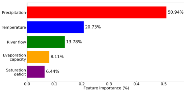
Fig. 5. Bar chart of feature importance values.
