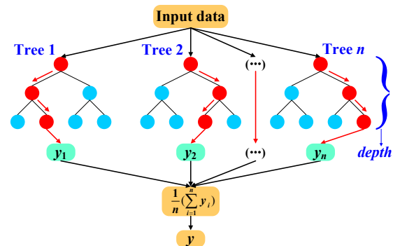
Fig. 1. Topology structure of random forest regression algorithm.
