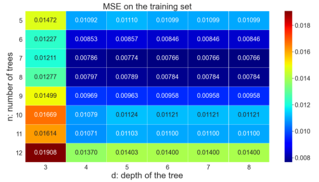
Fig. 4. MSE values of the training set with respect to different values of n (number of trees) and d (depth of the tree).
